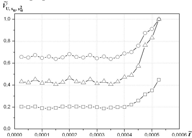
Fig. 3. Graphs of speed of change of amplitude parameters of AE resulting signal (Fig. 1) at the stages 1, 2 and elementary phase of the stage 3 in time in normalized units:
