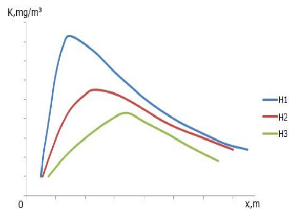
Fig. 3. Theoretical distribution of the concentration of impurities in air K at a distance x from a point source of different heights H : H1 < H2 < H3
