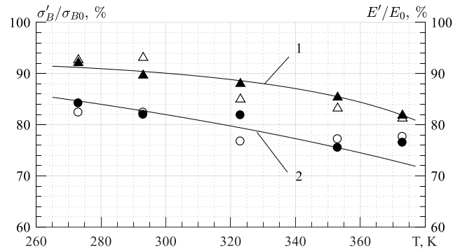
Fig. 1. Experimental (points) and calculated (curves) dependences of relative strength (●, 2) and relative elasticity modulus (▲, 1) of Twintex from temperature after exposure in AMg10 (light points) and seawater (dark points) for 120 hours
