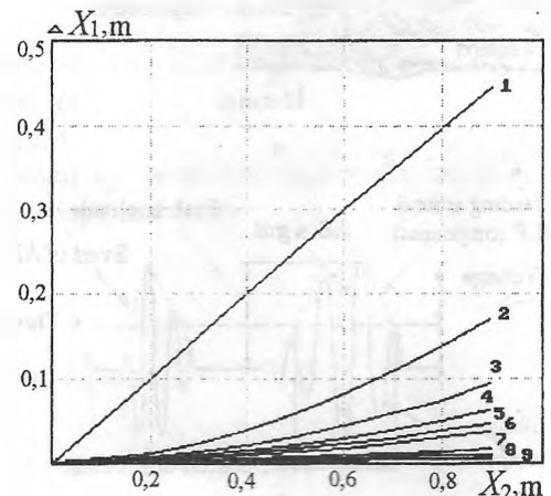
Fig. 4. Relationships showing the variation of the absolute value of the coordinate X_1 determination error as the function of the depth of the source of emission:
