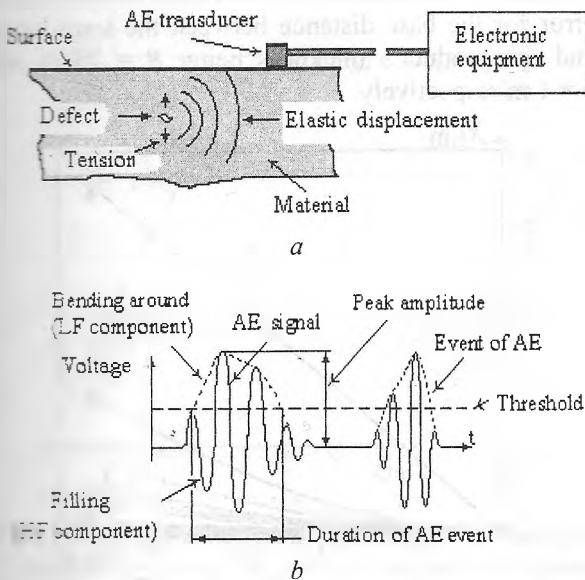
Fig. 1. AE signal radiation: a – detection of elastic displacement appearing when structural defects of the material develop under the influence of mechanical tensions; b – AE signal parameters under processing
