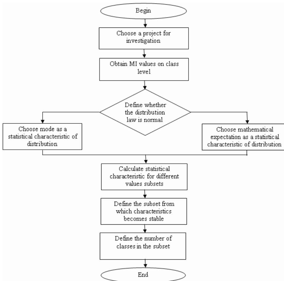
Fig.1 Algorithm scheme
