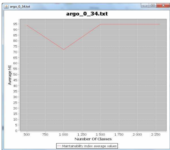
Fig.6 Investigation of AgroUML 3.0.4
