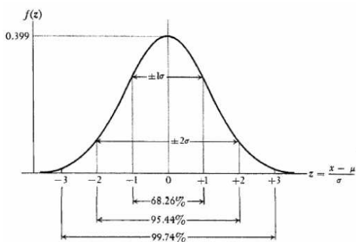
Fig.3 Normal distribution
