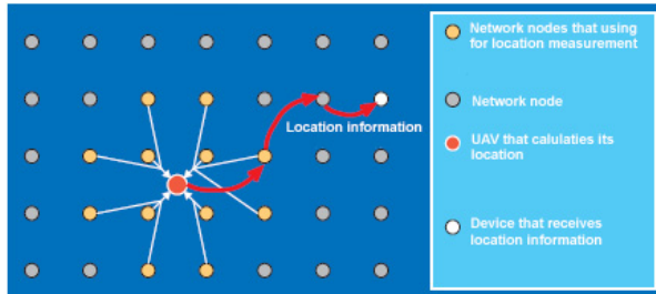
Fig. 2. ZigBee network with messaging and positioning capabilities
