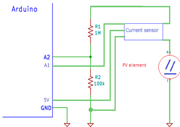
Fig. 1. Lower level system main circuit
