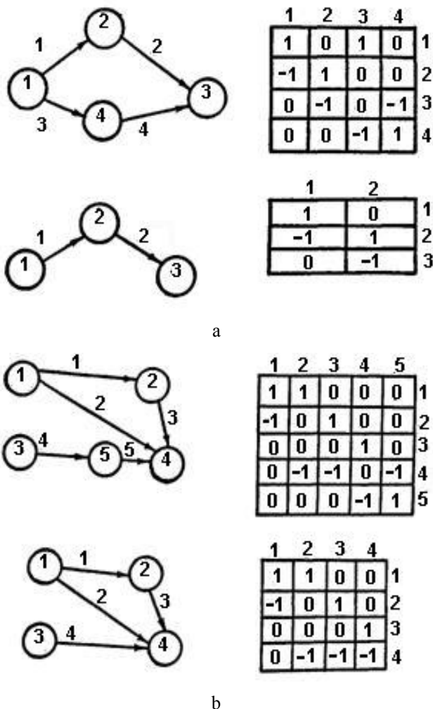
Fig. 3. Rules of transformation of the oriented graph for measuring (a) and converting (b) devices
