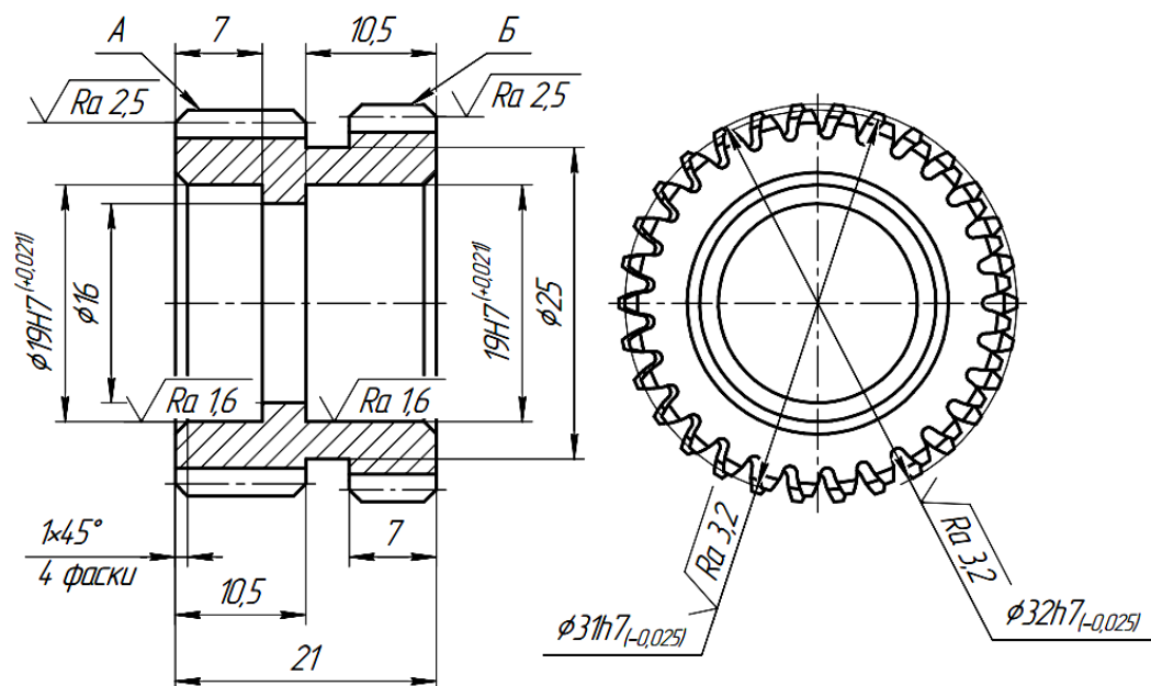
Fig. 1. Drawing of a block of gears
