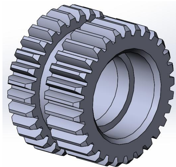
Fig. 2. Solid-state model of the gear blockper
